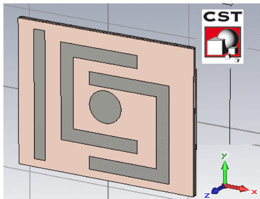
Fig 4. Rectangular microstrip patch antenna with desired metamaterial structure.
