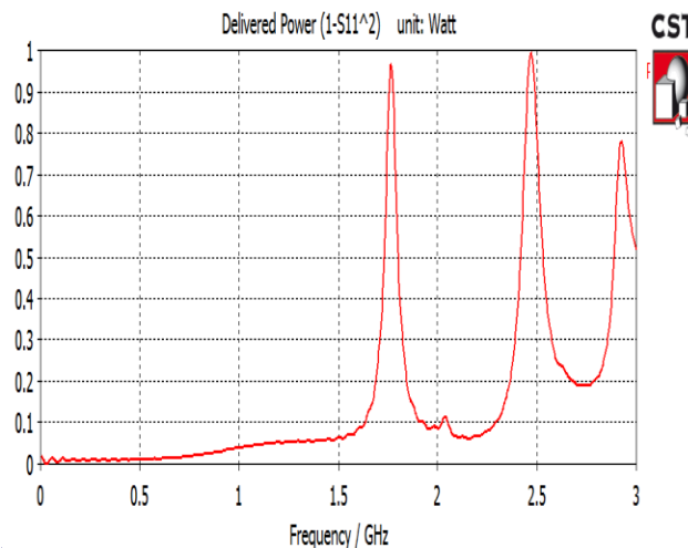
Fig 9. Delivered power to reduced size RMPA loaded with metamaterial structure
