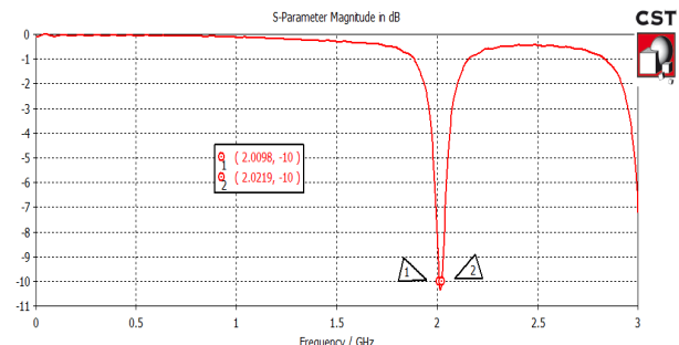
Fig 2. Simulation of return loss and bandwidth of RMPA alone.
