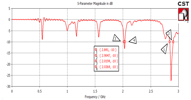
Fig 5. Simulation results of Return loss and impedance bandwidth of RMPA with desired metamaterial structure at 2.865 GHz.
