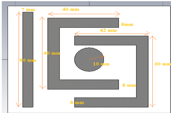
Fig 3. Design of desired metamaterial structure at the height of 3.2 mm from ground plane.
