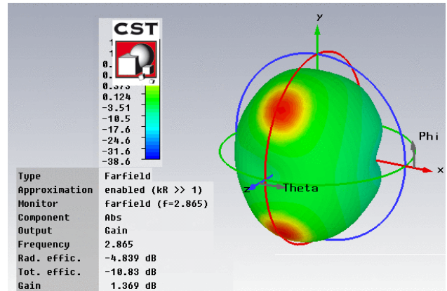
Figure11. gain of the RMPA alone at 2.865 GHz.
