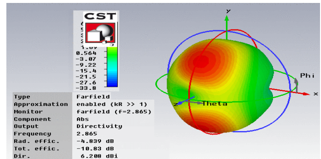
Fig 6. Radiation pattern of RMPA at dual band operation.
