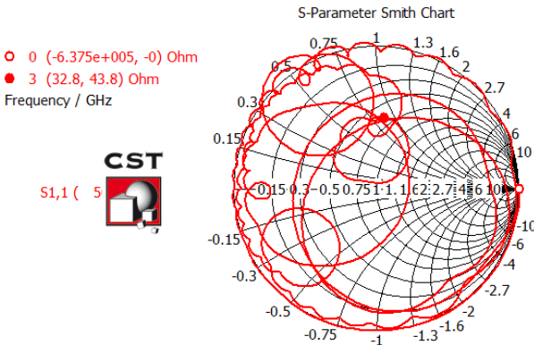
Figure 15. Smith chart of PMPA loaded with metamaterial
