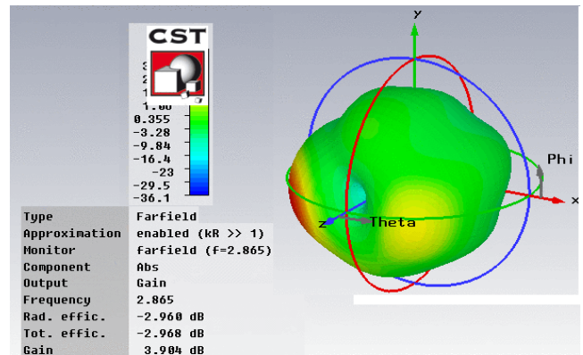
Figure12. gain of the RMPA alone at 2.865 GHz .
