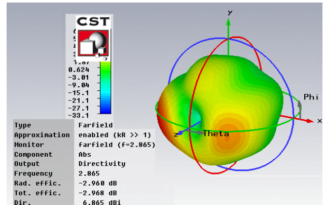
Fig 7. Radiation pattern of desired antenna showing Directivity of 6.865 dBi.
