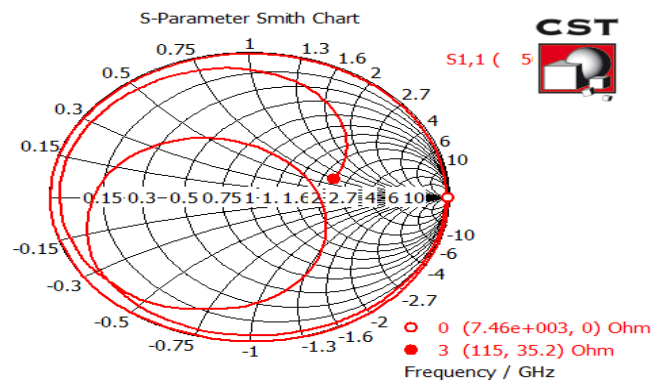
Figure 14. Smith chart of simple Rectangular microstrip patch antenna at operating frequency.
