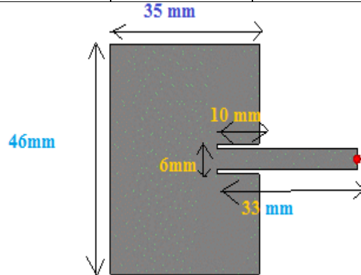
Fig 1: Rectangular microstrip patch antenna(RMPA) designed at 1.764GHz & 2.472 GHz.
